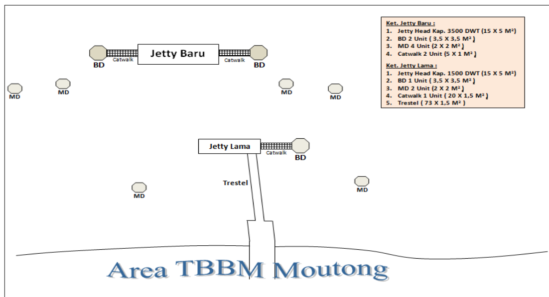
Figure 2 – Layout of Jetty I ( 3500 DWT)
