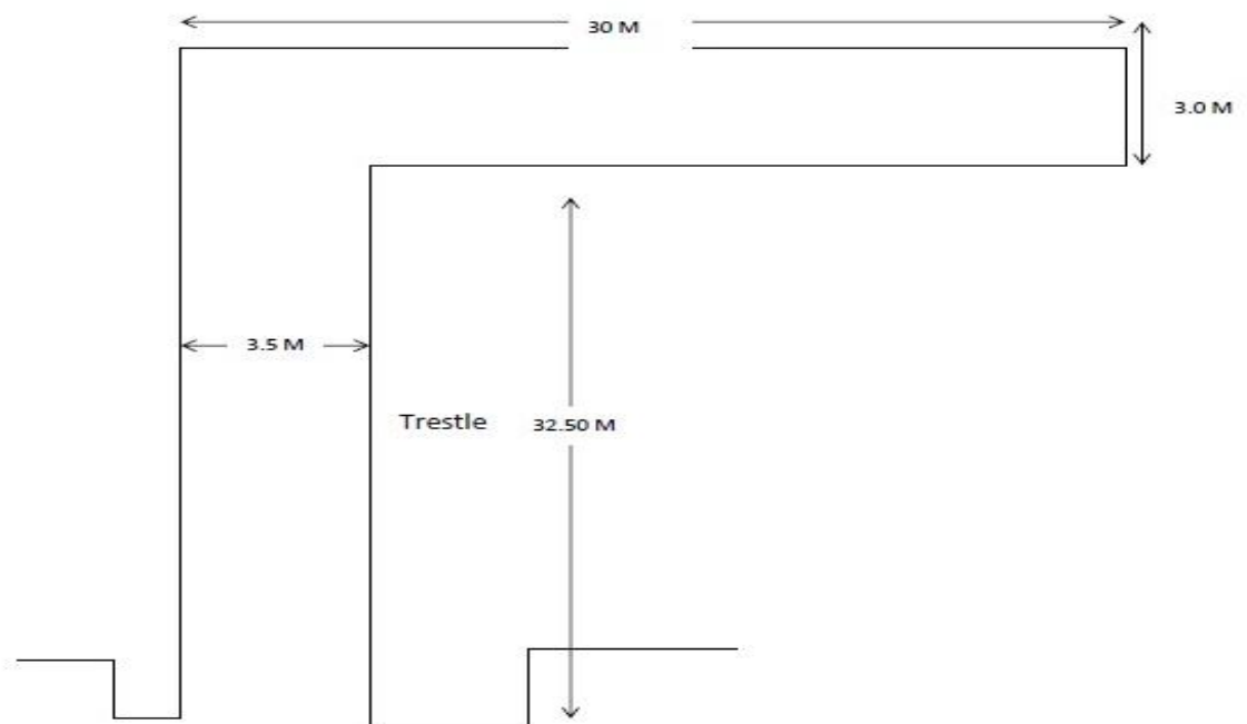
Figure 3 – Layout Jetty III ( 750 DWT)
