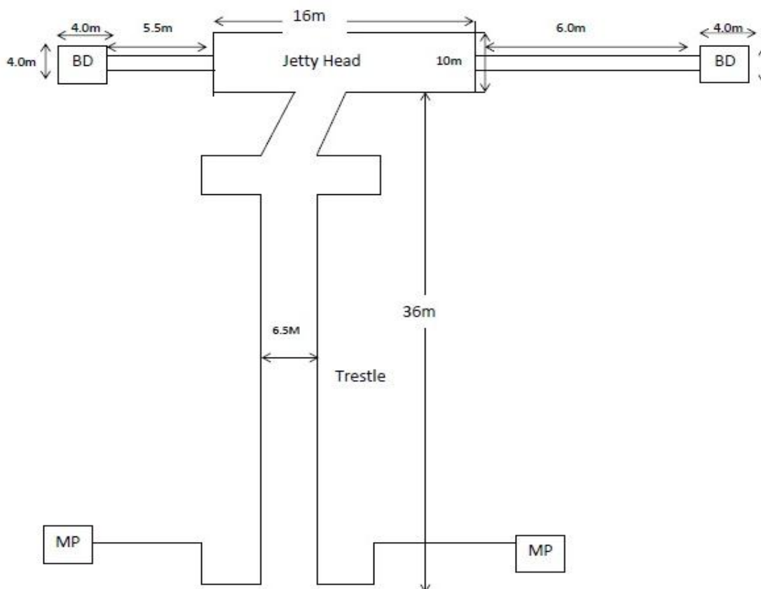
Figure 1 – Layout Jetty I ( 17500 DWT)
