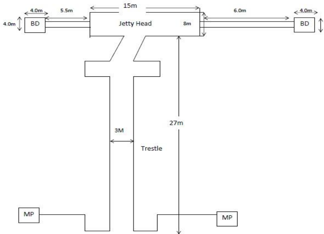
Figure 2 – Layout Jetty II ( 6500 DWT)
