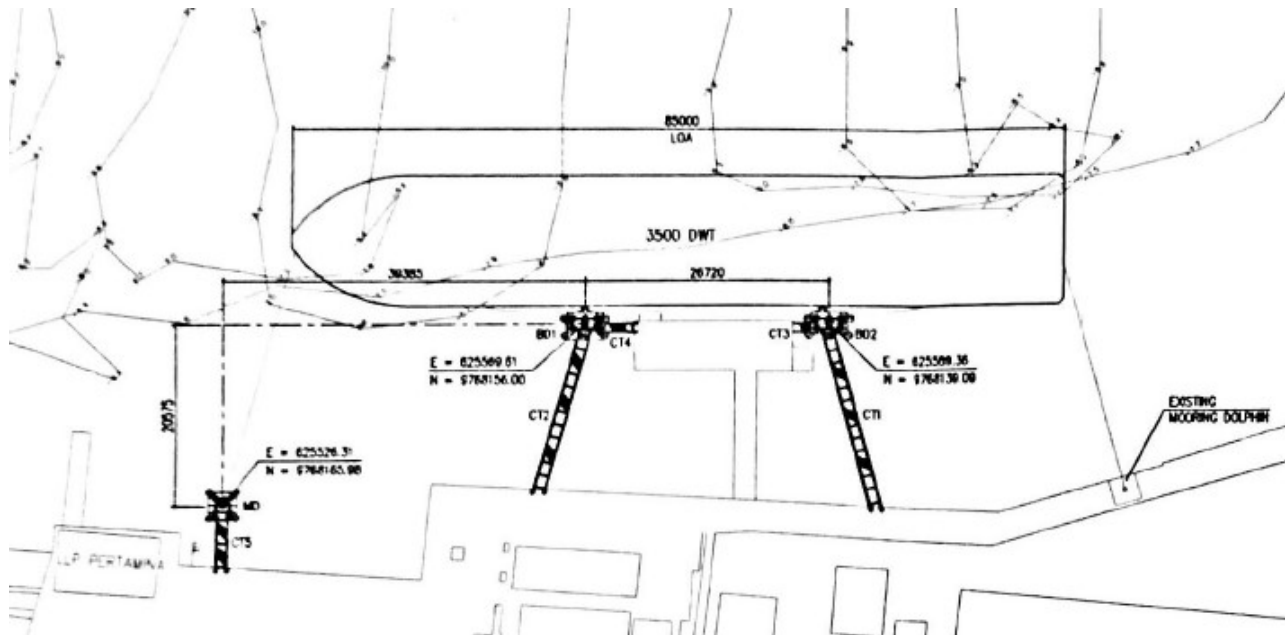
Gambar 1.1 – Layout Jetty Pangkal Balam
