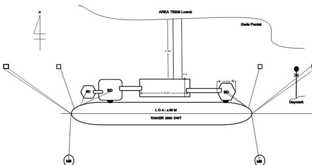
Figure 1 – Layout of Jetty
