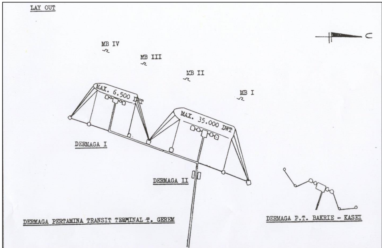
Gambar 1.2 - Layout Jetty I & II Tanjung Gerem
