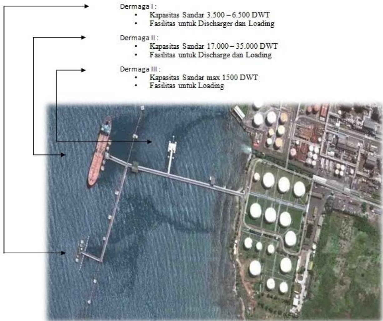
Gambar 1.1 - Layout Jetty I & II Tanjung Gerem
